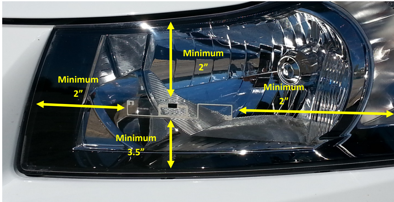
Clearance Shown for Distance between Hood, Body Panel & Bumper
